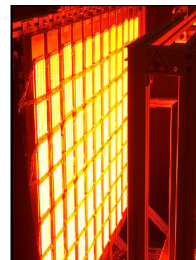
Large LED Simulator Illuminating Solar Panels
