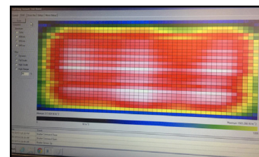
Snapshot of beam scanner output from LARGE (1.2 m 2 ) solar simulator AFTER optimizing the intensity distribution of the LEDs.
